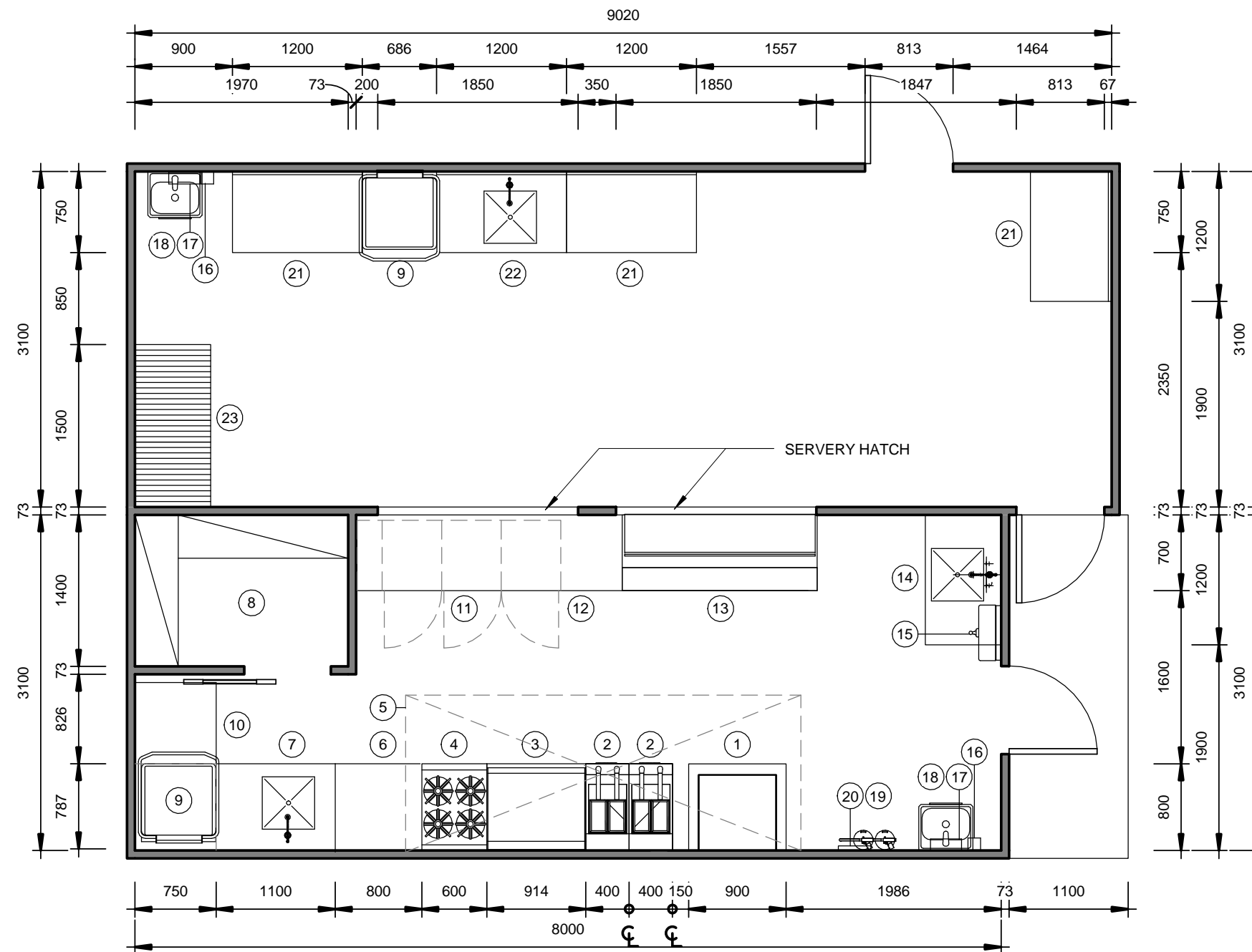
1 Proposed Floor Plan 1 : 50
